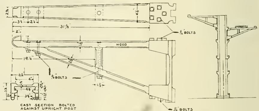
PAINT SHOP SCAFFOLDING, PENNSYLVANIA LINES.
